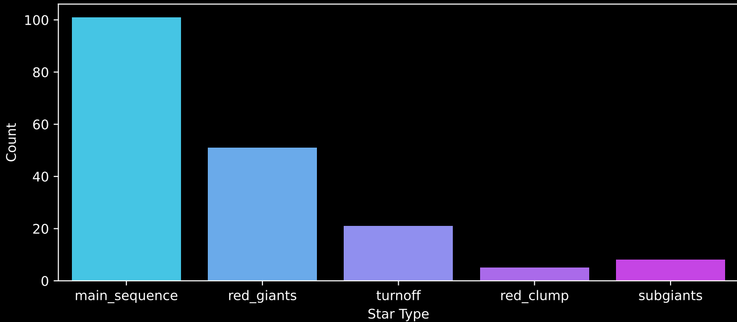
APOGEE DR17 Field: [151-45_MGA] Count plot of Star Type
