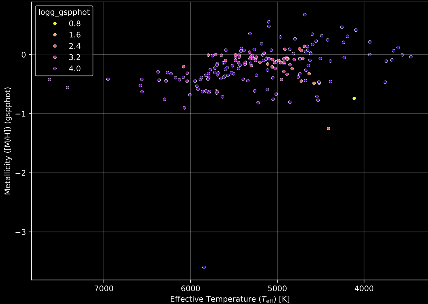
APOGEE DR17 Field: [151-45_MGA] Stellar Population Parameters (n= 186)
