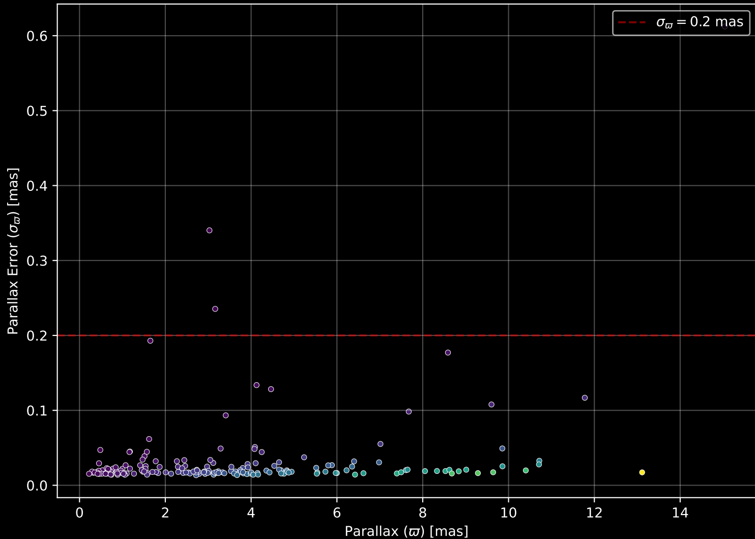
APOGEE DR17 Field: [151-45_MGA] Parallax Quality (n= 186)
