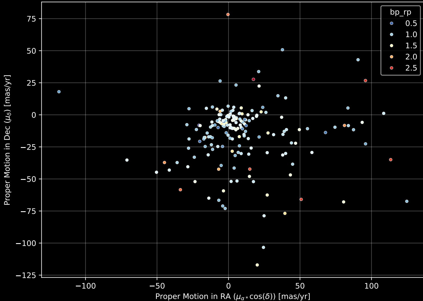
APOGEE DR17 Field: [151-45_MGA] Proper Motion Diagram (n= 186)
