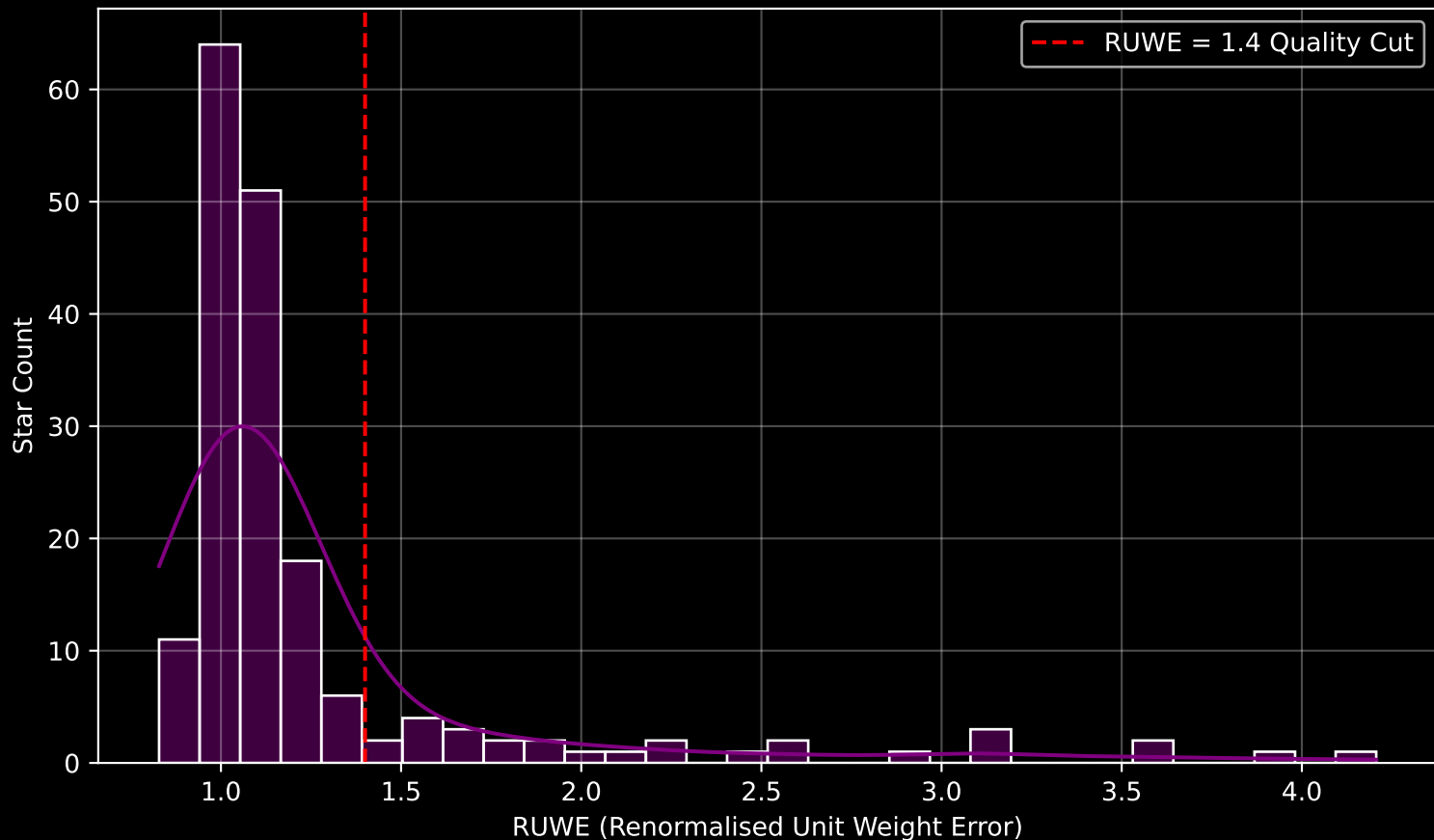
GAPOGEE DR17 Field [151-45_MGA] RUWE Distribution (n= 178)
