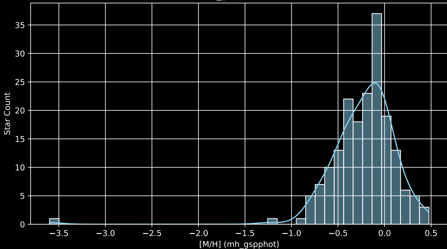
APOGEE DR17 Field: [151-45_MGA [M/H] (mh_gspphot) (n= 184)
